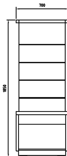
FRONTAL CMCT-70-RC
